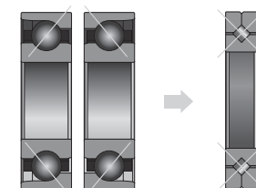
Traditional Ball bearing
