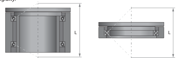
Traditional Ball bearing combination space
