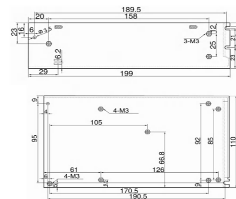
LSP-260-24, LSP-360-24
