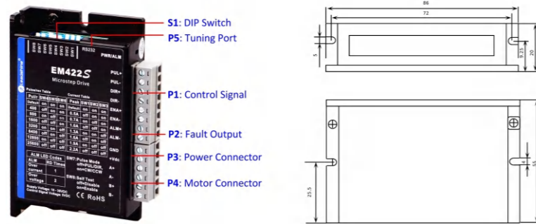
EM415S, EM422S
