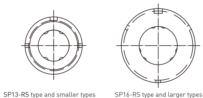
Figure 7-2 Position of the spline groove for RS type
