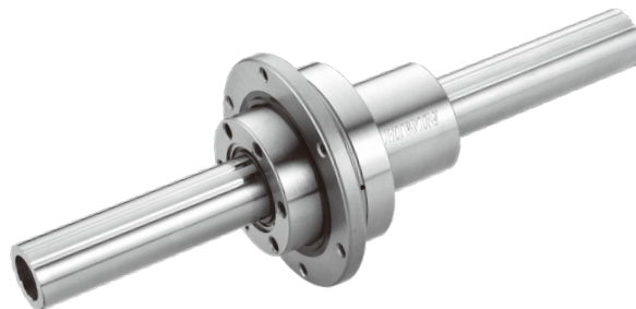
(3) Rotary type (FSR type)
